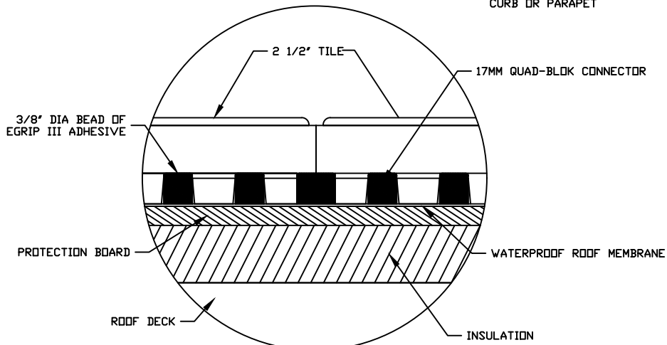
DETAIL "A"
